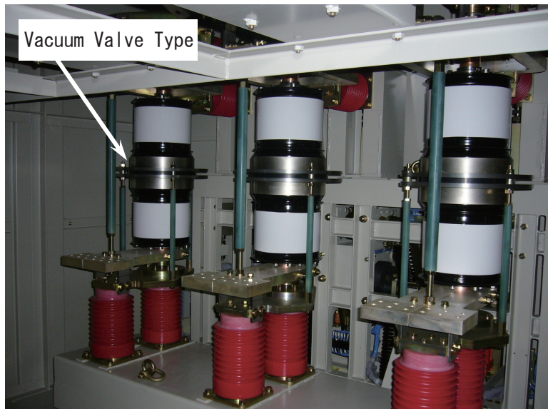
Photo Back-up circuit breakers renewed (vacuum valve type)
